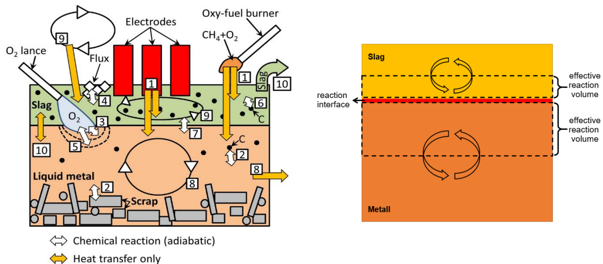
Fig. 1. Development of an Electric Arc Furnace Simulation Model Using the EERZ Approach
