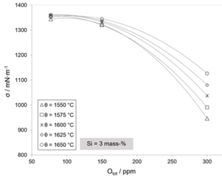
6. Figure 1: Surface tension of liquid electrical steel as a function of total oxygen content for different temperatures with a silicon concentration of 3 mass-% [4]
