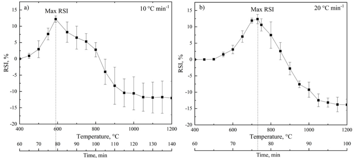
Figure 1. RSI changes during heating by H 2 under different heating rate
