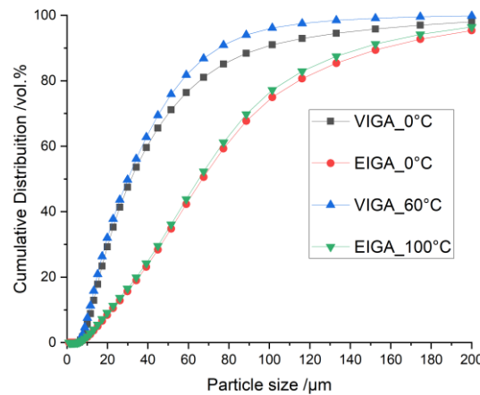
Figure 1: Comparison of the particle size distribution between VIGA and EIGA at different gas preheating temperatures.
