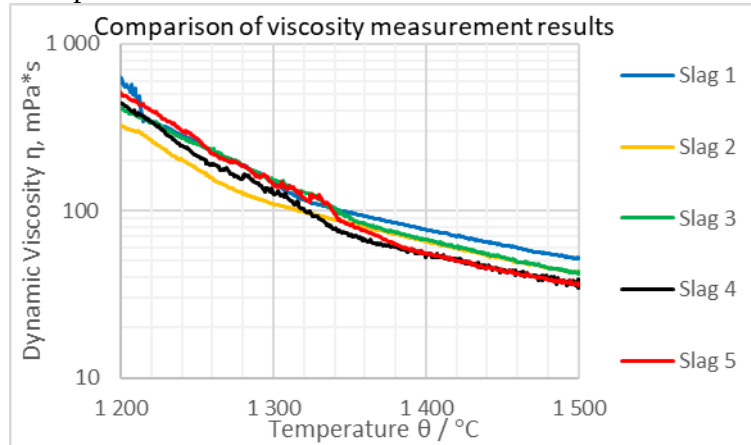
Figure 1: Temperature function of viscosity of slags with different cobalt oxide contents
