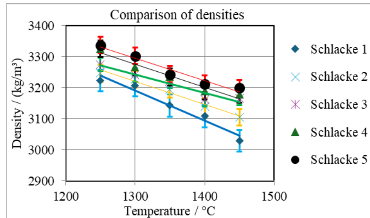
Figure 2: Temperature function of density of slags with different cobalt oxide contents
