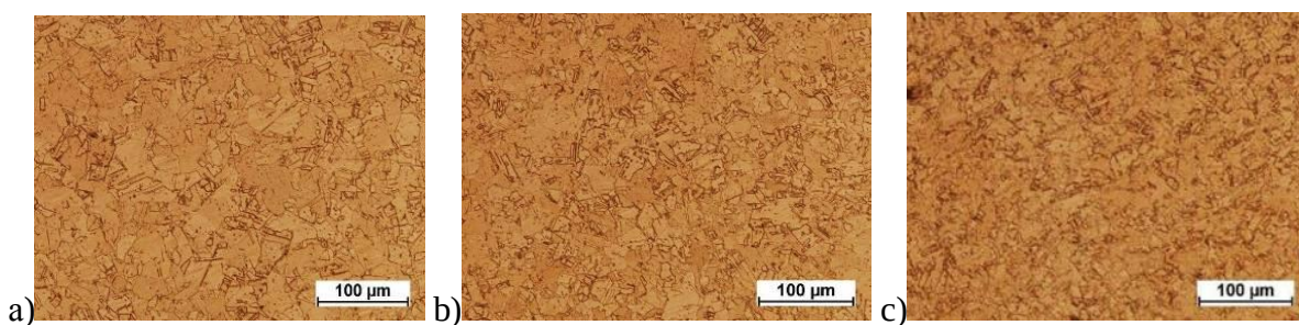
Figure 2 – Copper microstructures after 4 passes of deformation on a radial-shear rolling mill at temperatures: a) 200°C, b) 100°C, c) 20°C
