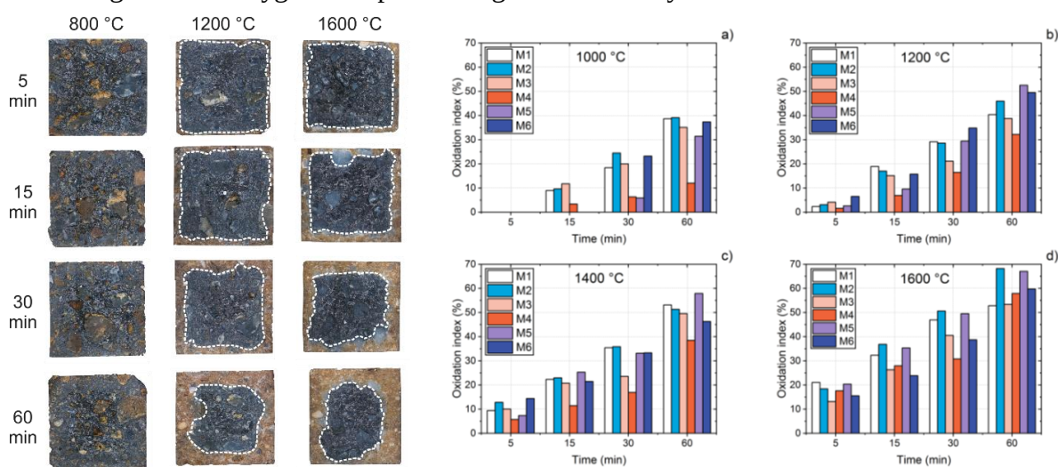
Figures II: a) Cross-sectional analysis of M1 sample (20 × 20 mm) after oxidation at 800, 1200, and 1600 °C for holding times of 5, 15, 30, and 60 min [1] ; b) Oxidation index of MgO–C samples during oxidation at different holding times: a) 1000 °C; b) 1200 °C; c)
