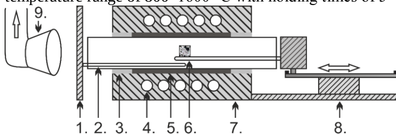
Figure I. Schematic view of the open high-temperature microscope. 1. Protective wall; 2. Pt-Rh thermoelement; 3. Insulator; 4. Inductor; 5. Carbon heat element; 6. Sample on corundum holders; 7. Furnace body (alumina); 8. Sample entry mechanism; 9. Ventilation.
